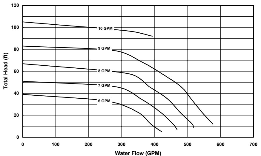
SM50 Pump Performance
